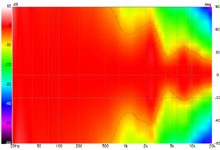
HORN DIRECTIVITY
