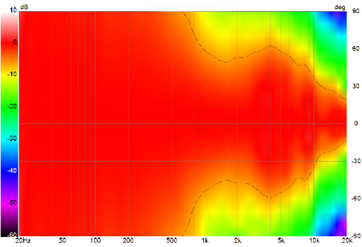
COLLAR DIRECTIVITY
