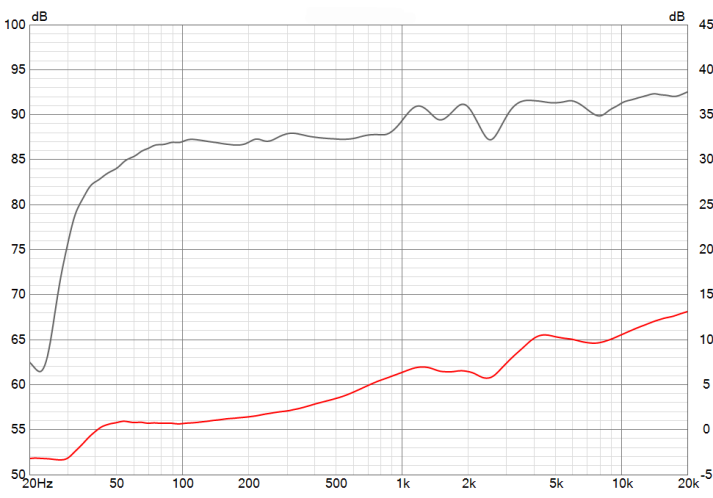
HORN SPL
