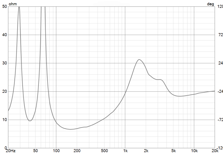
HORN IMPEDANCE
